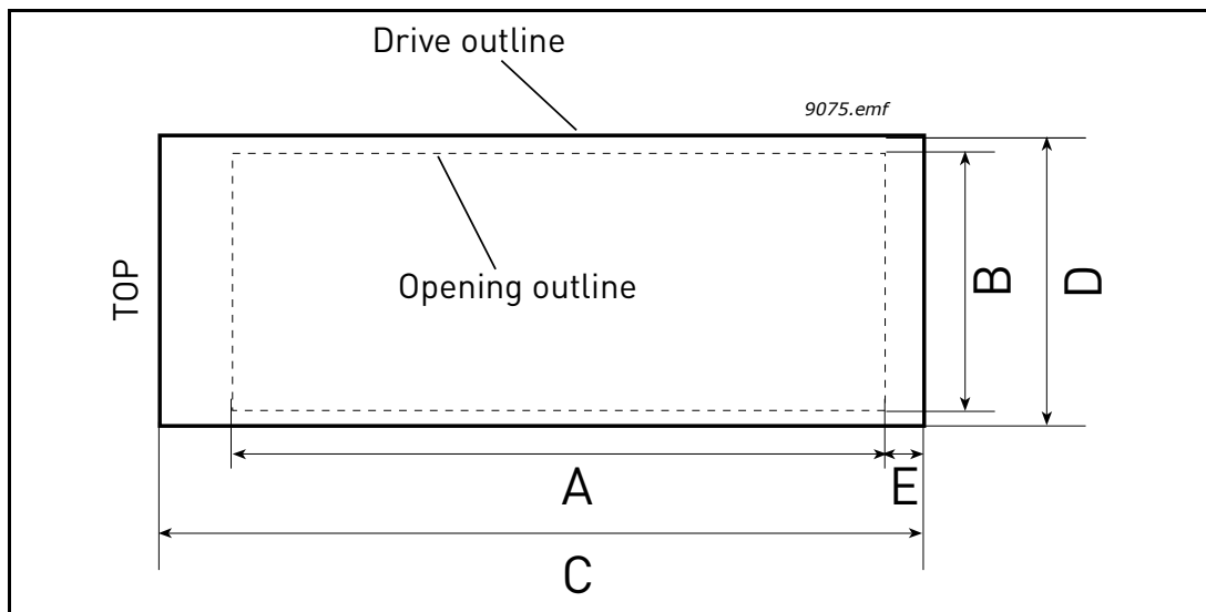
Figure 13. Flange mount cutout dimensions for MR7 to MR9
