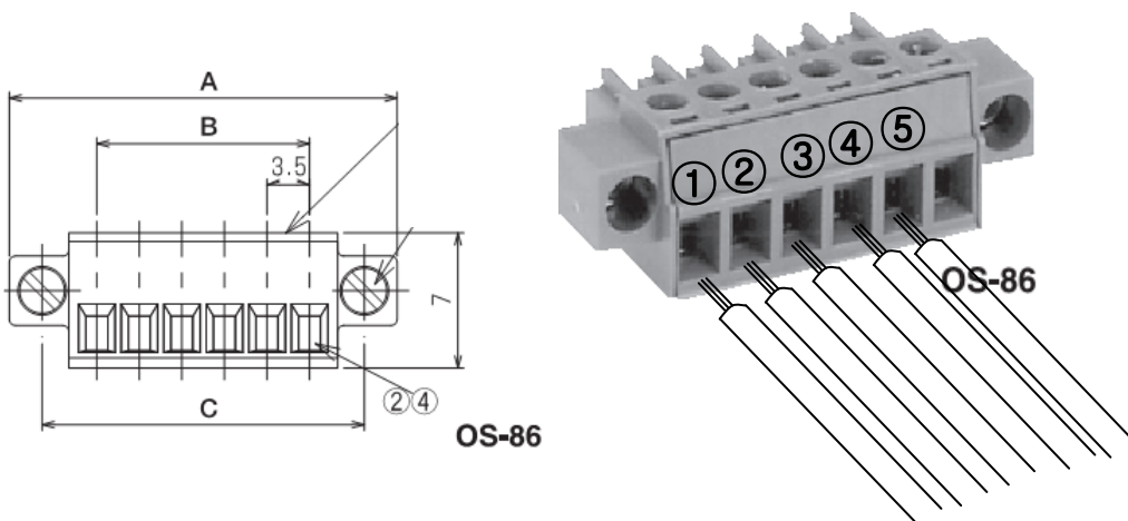
<Connector Structure>
