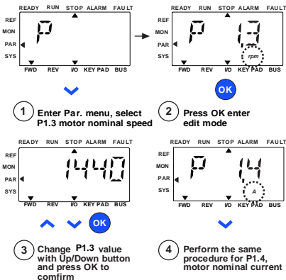
Figure 2: Vacon 10 startup wizard (standard application)
