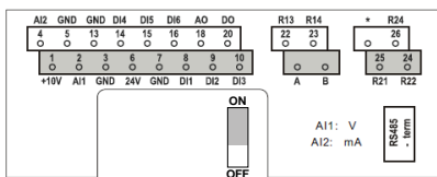
Figure 3.1: Vacon 10 I / O
