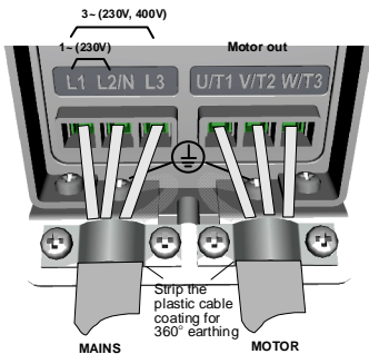
Figure 4: Vacon 10 power connections, M11
