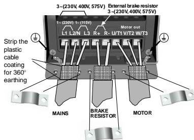
Figure 5: Vacon 10 power connections, M12 - M13
