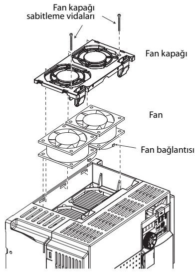
FR-E740-120SC örneği
