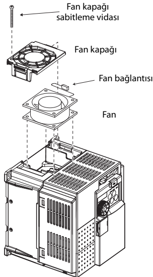
FR-E740-095SC örneği
